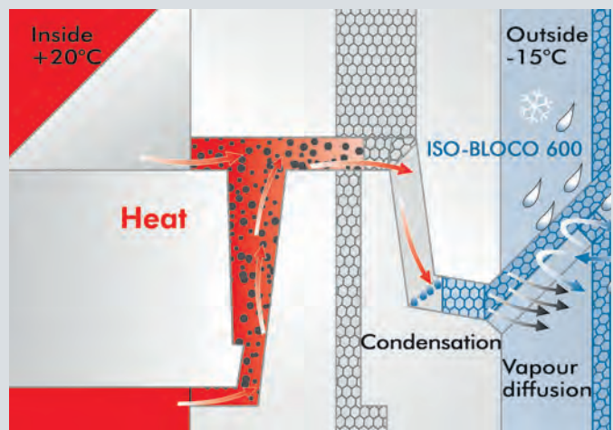
ISO-BLOCO 600 ensures sealing against wind and rain up to 600Pa and allows condensation to diffuse through the facade joint.
