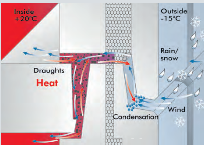
Warm internal air escapes through the joints and condenses on the cold surface. This results in draughts and damage to the building.
